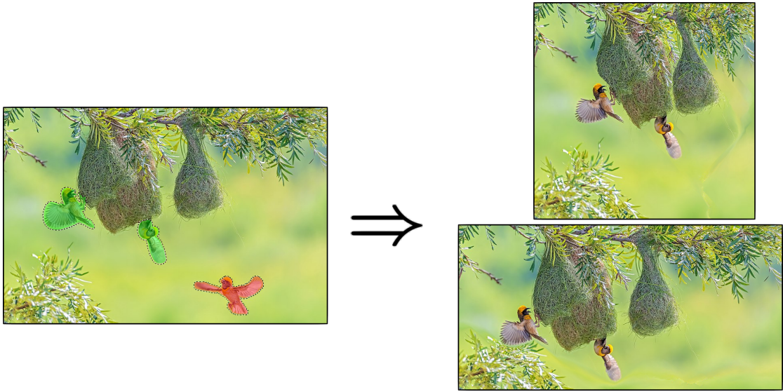
Figure 1: Vertical and horizontal seam carving of an image with a mask: we remove the bottom right bird and keep the two other.
